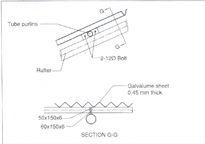
FIG: PURLIN TO RAFTER CONNECTION
